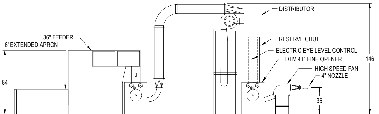
SYSTEM II w/DOUBLE NOZZLE
